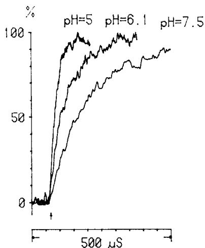
Fig.2. The effect of pH on the kinetics of the \Delta\psi generation phase with \tau \sim 0.1 – 0.2 ms, induced by the second flash. Each curve is derived by subtracting the curve induced by the second flash from that induced by the first flash and normalized to 100%.
